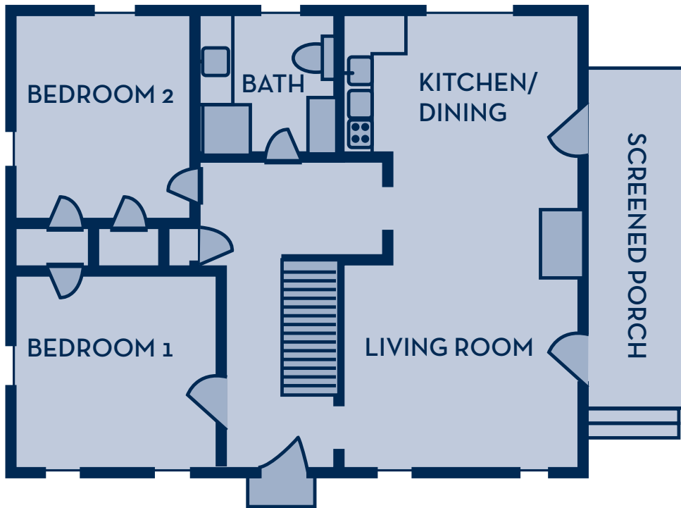
First floor: Living room, kitchen/dining, bedroom 1 (one queen bed), bedroom 2 (two single beds).
